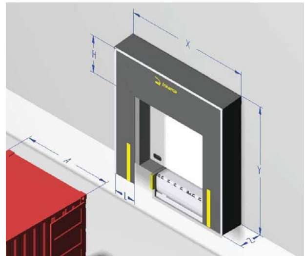
Shelter with 10% slope for draining water.
